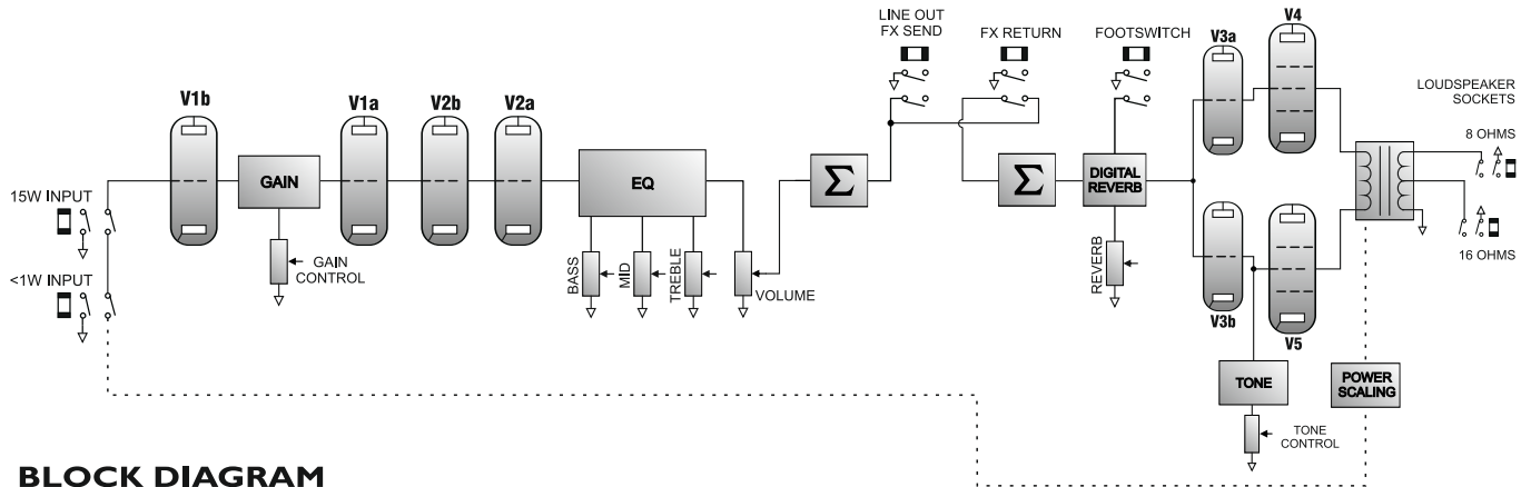
BLOCK DIAGRAM
